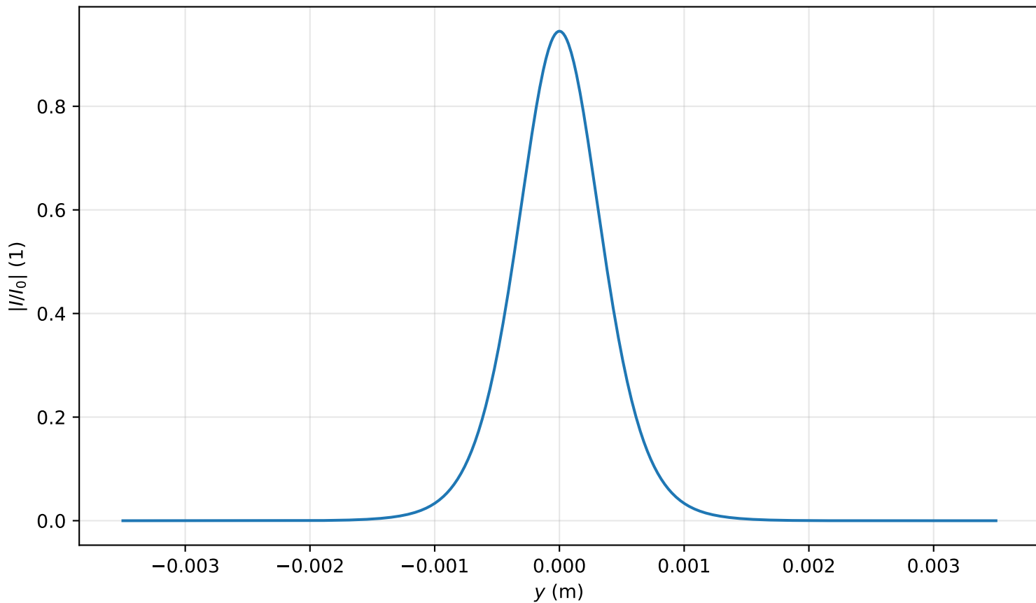
Intensity profile I(x = 0, y, z = 1.990)/I_0 , P_{in}=0.6P_{cr} , artificial time
